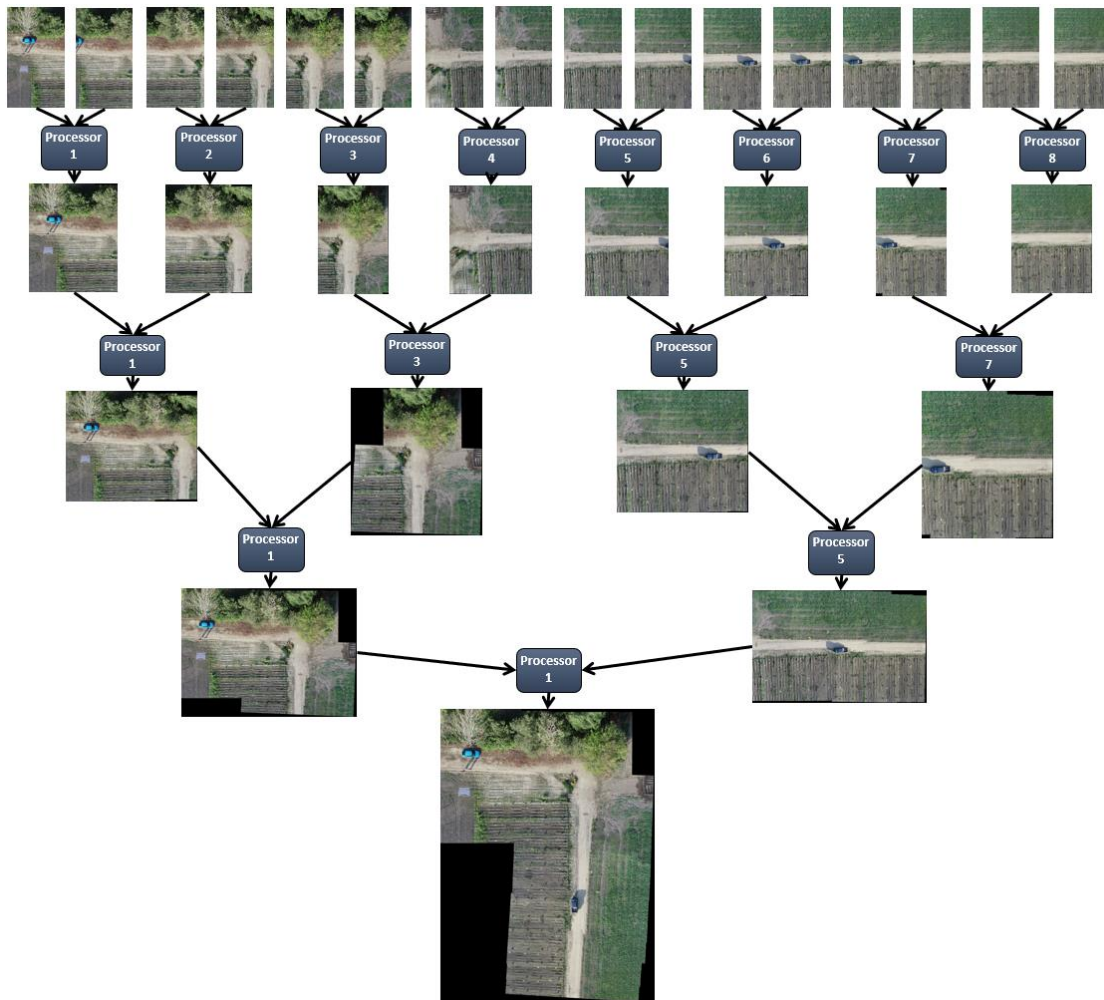
Fig. 5 Tree-based image fusion algorithm.
