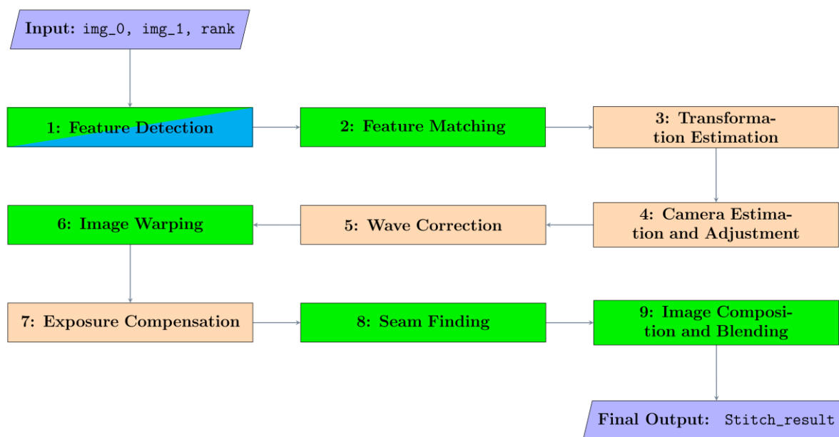
Fig. 3 Image stitching workflow.
